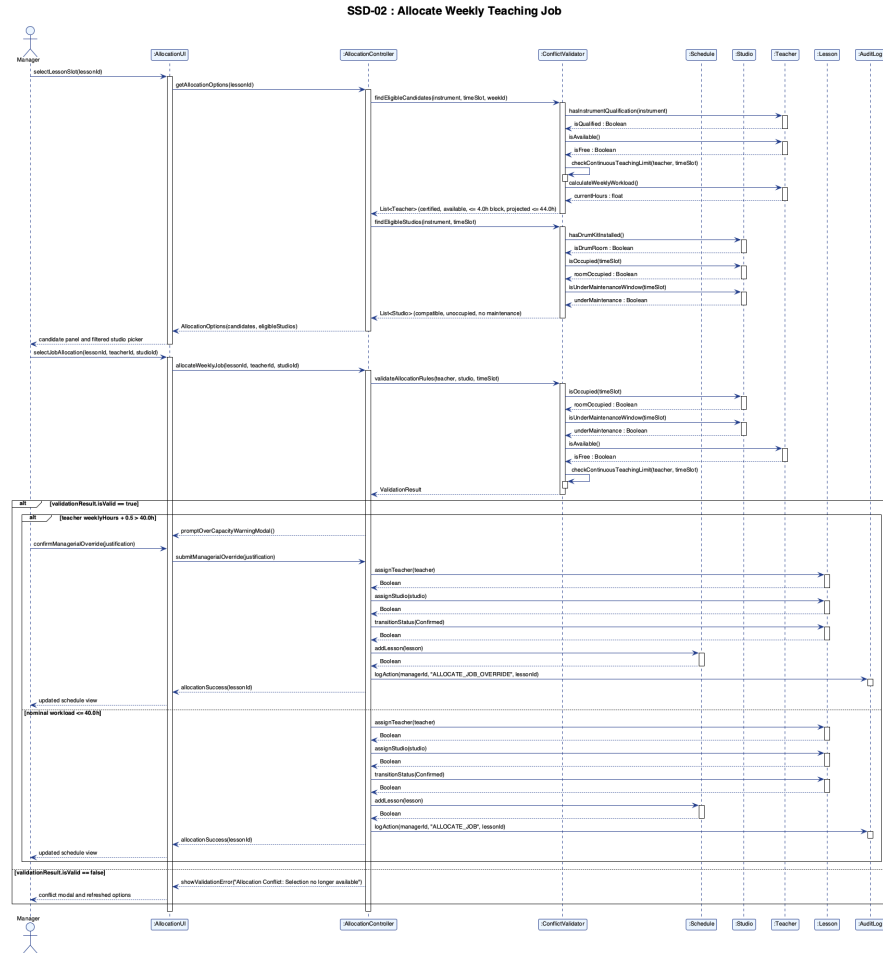
Figure 4.4: SSD-02 Allocate Weekly Teaching Job
