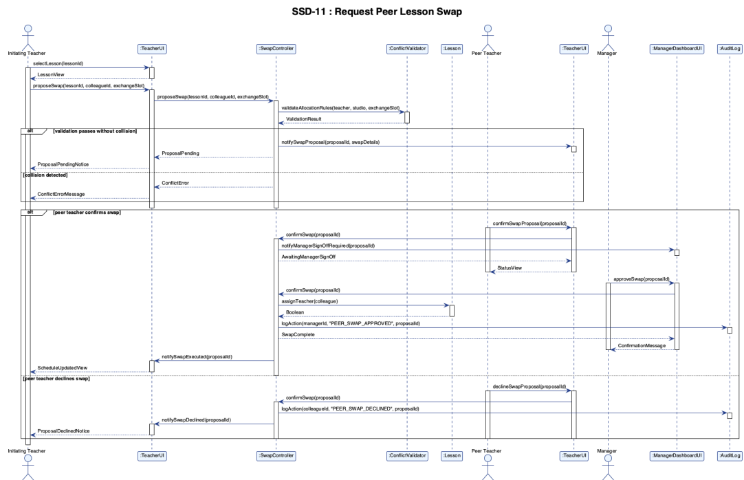
Figure 4.13: SSD-11 Request Peer Lesson Swap
