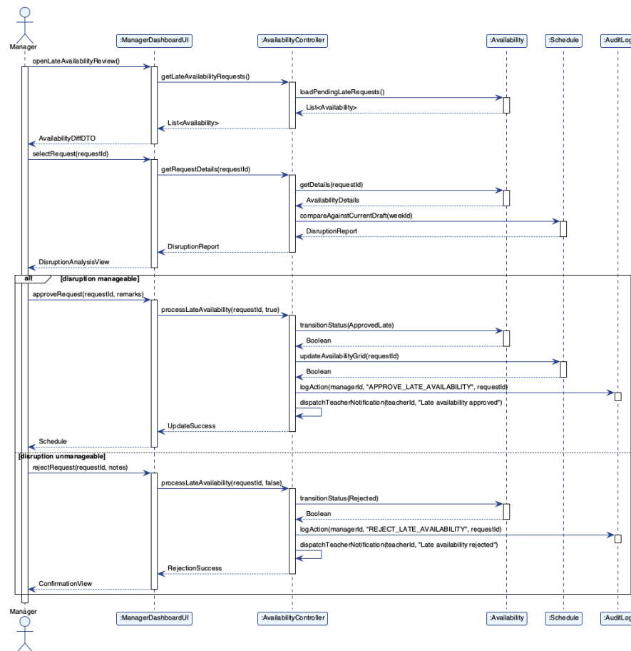
Figure 4.6: SSD-04 Process Late Availability Exception
