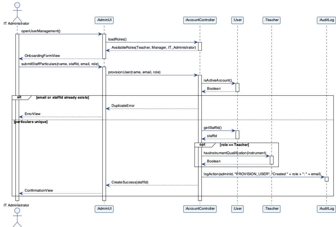
Figure 4.14: SSD-12 Onboard New Staff & Manager Accounts
