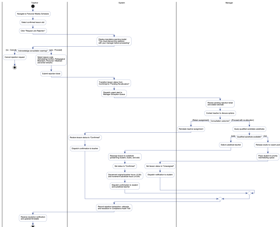
Figure 3.3: Activity Diagram for 2-Stage Job Rejection Workflow
