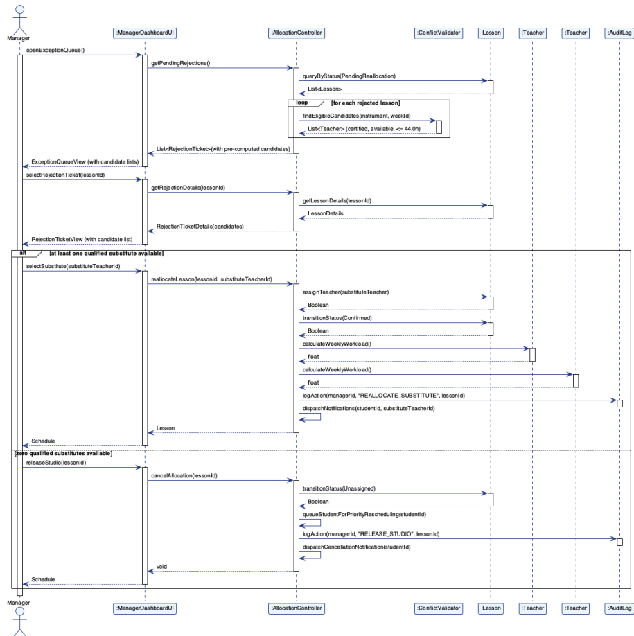
Figure 4.5: SSD-03 Review & Re-allocate Rejected Lesson
