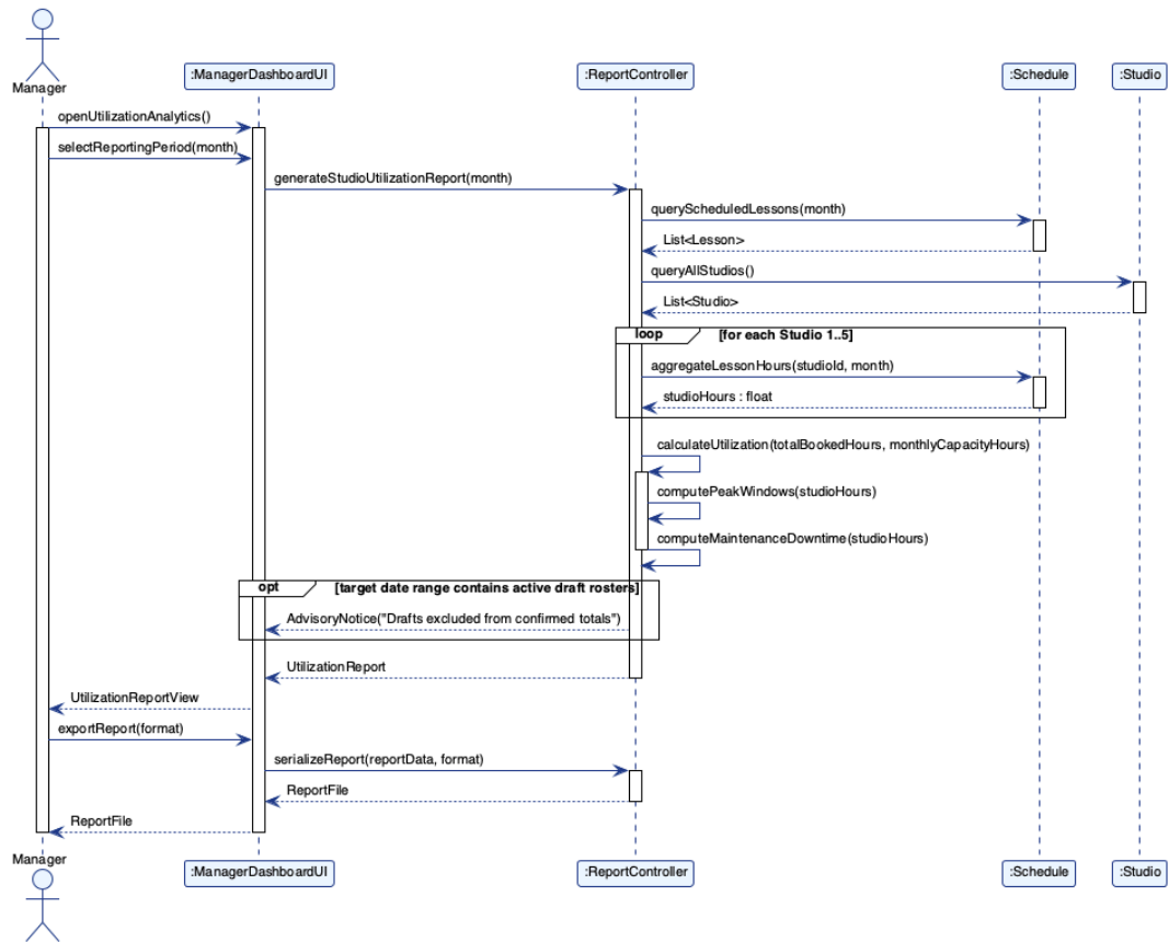
Figure 4.18: SSD-16 Generate Studio Utilization Report
