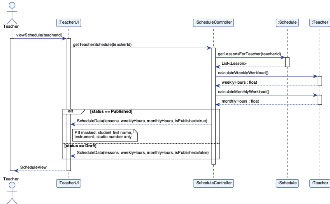
Figure 4.11: SSD-09 View Confirmed Schedule & Workload
