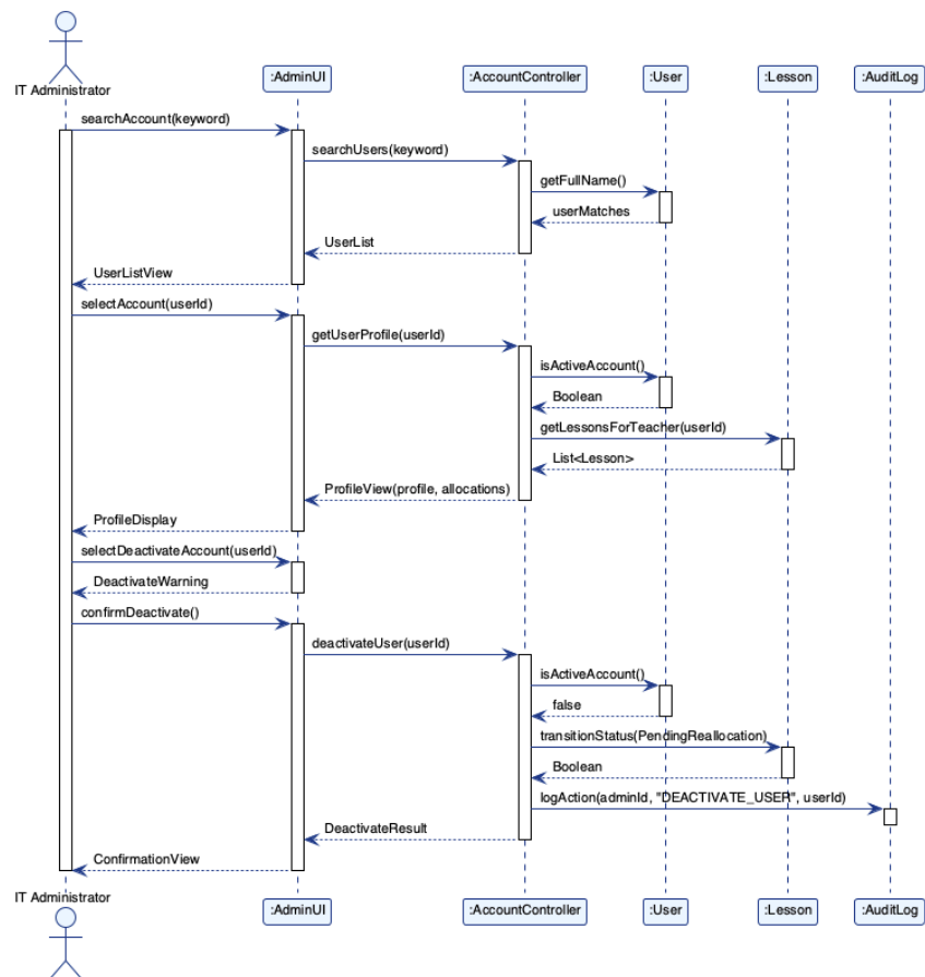
Figure 4.15: SSD-13 Manage User Account Status & Access
