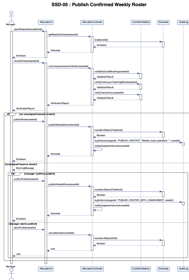
Figure 4.7: SSD-05 Publish Confirmed Weekly Roster
