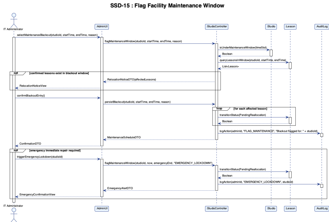
Figure 4.17: SSD-15 Flag Facility Maintenance Window
