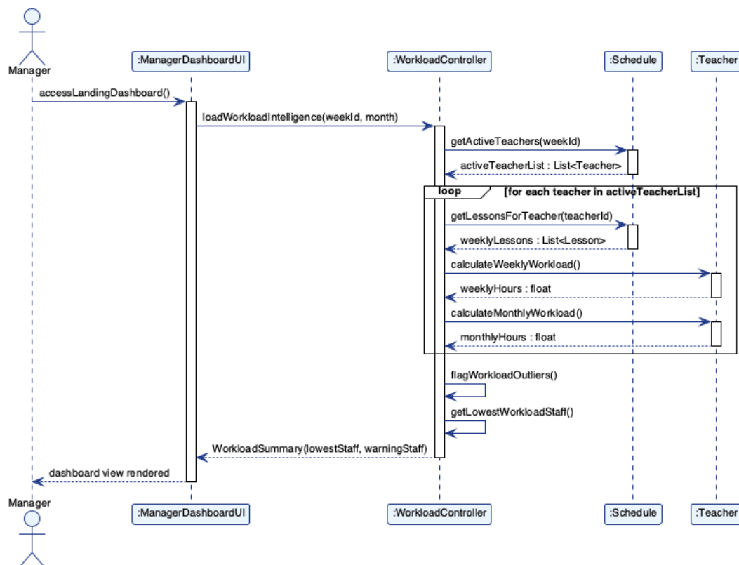
Figure 4.3: SSD-01 View Workload Dashboard & Outliers
