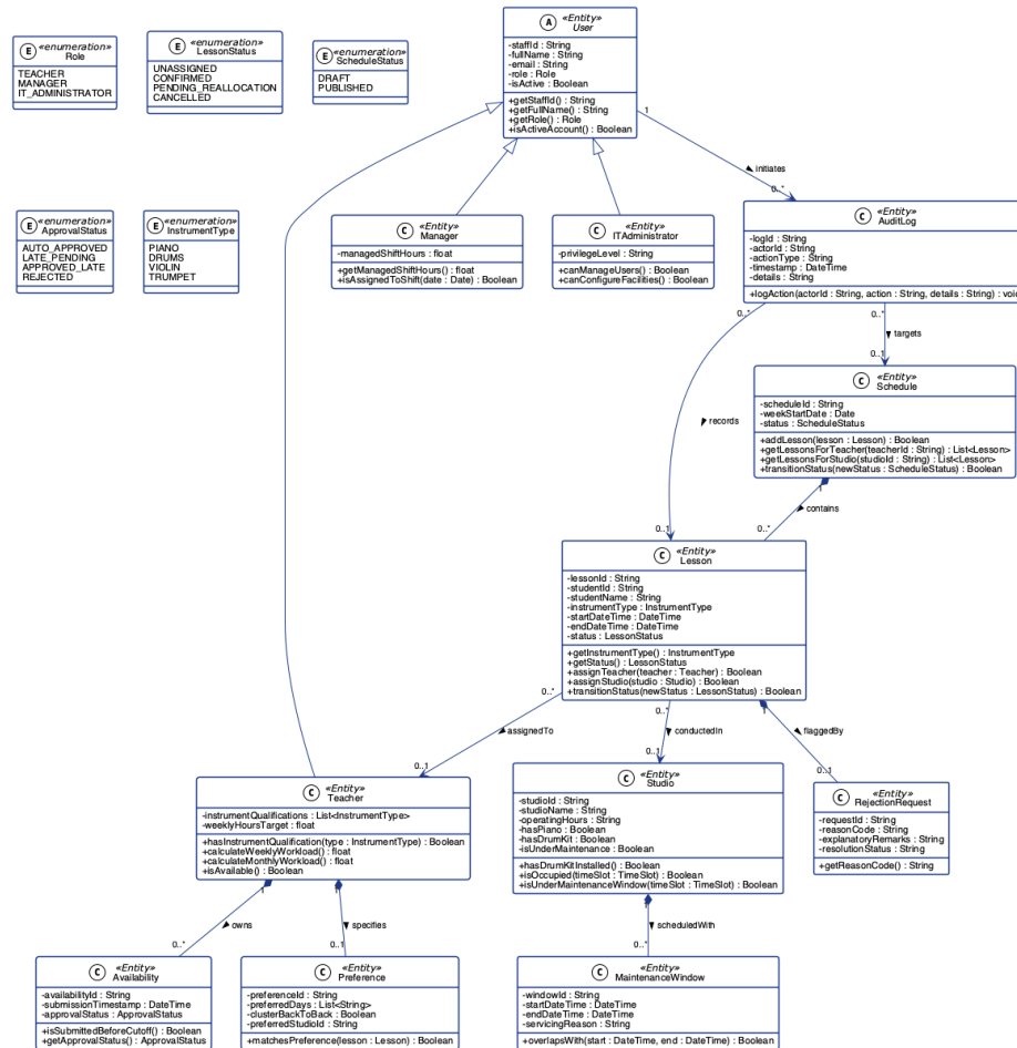
Figure 4.1: Domain Entity Class Diagram (Inheritance, Compositions, Associations & Enums)
