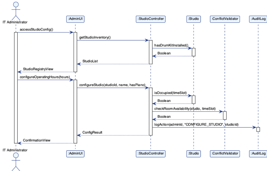
Figure 4.16: SSD-14 Configure Studio & Instrument Setup
