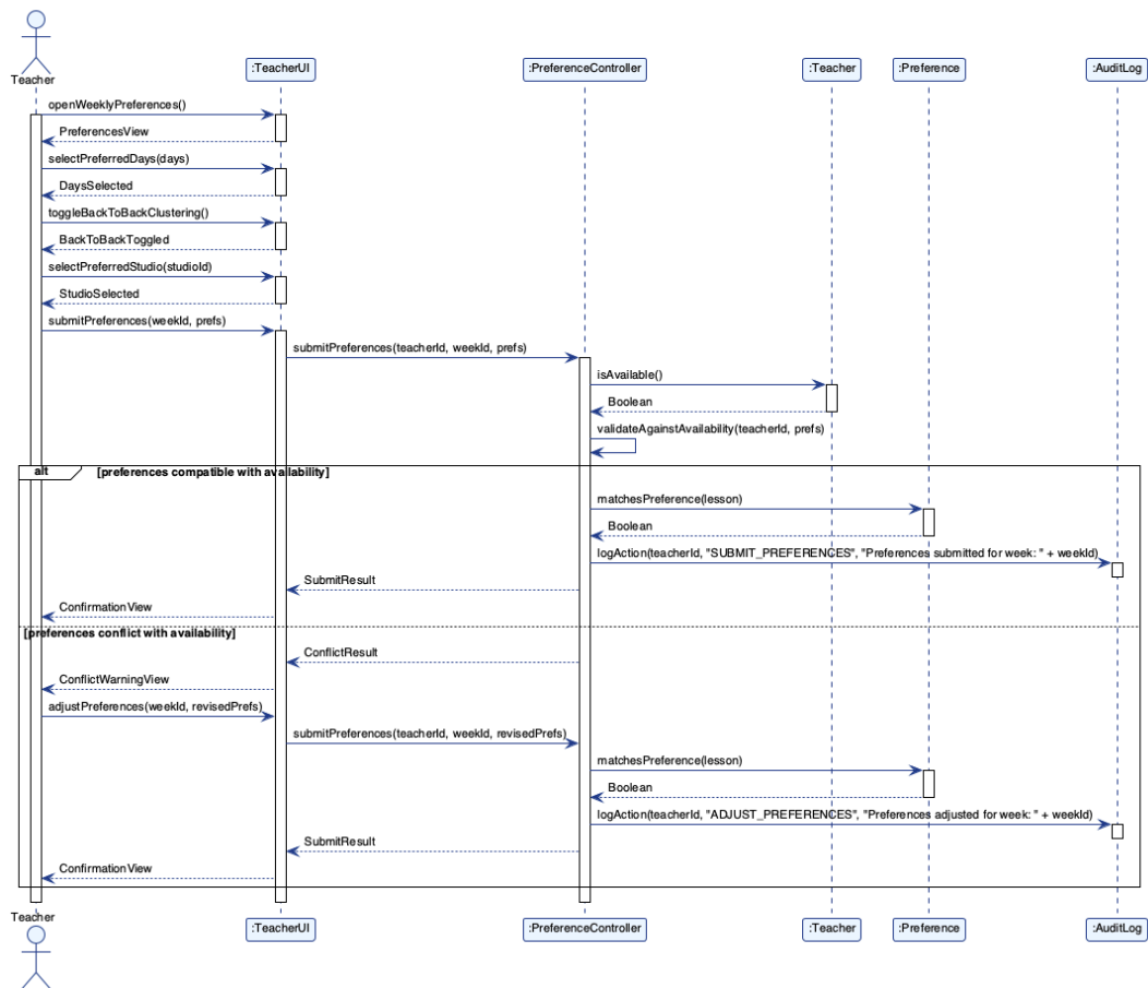
Figure 4.10: SSD-08 Submit Weekly Job Preferences
