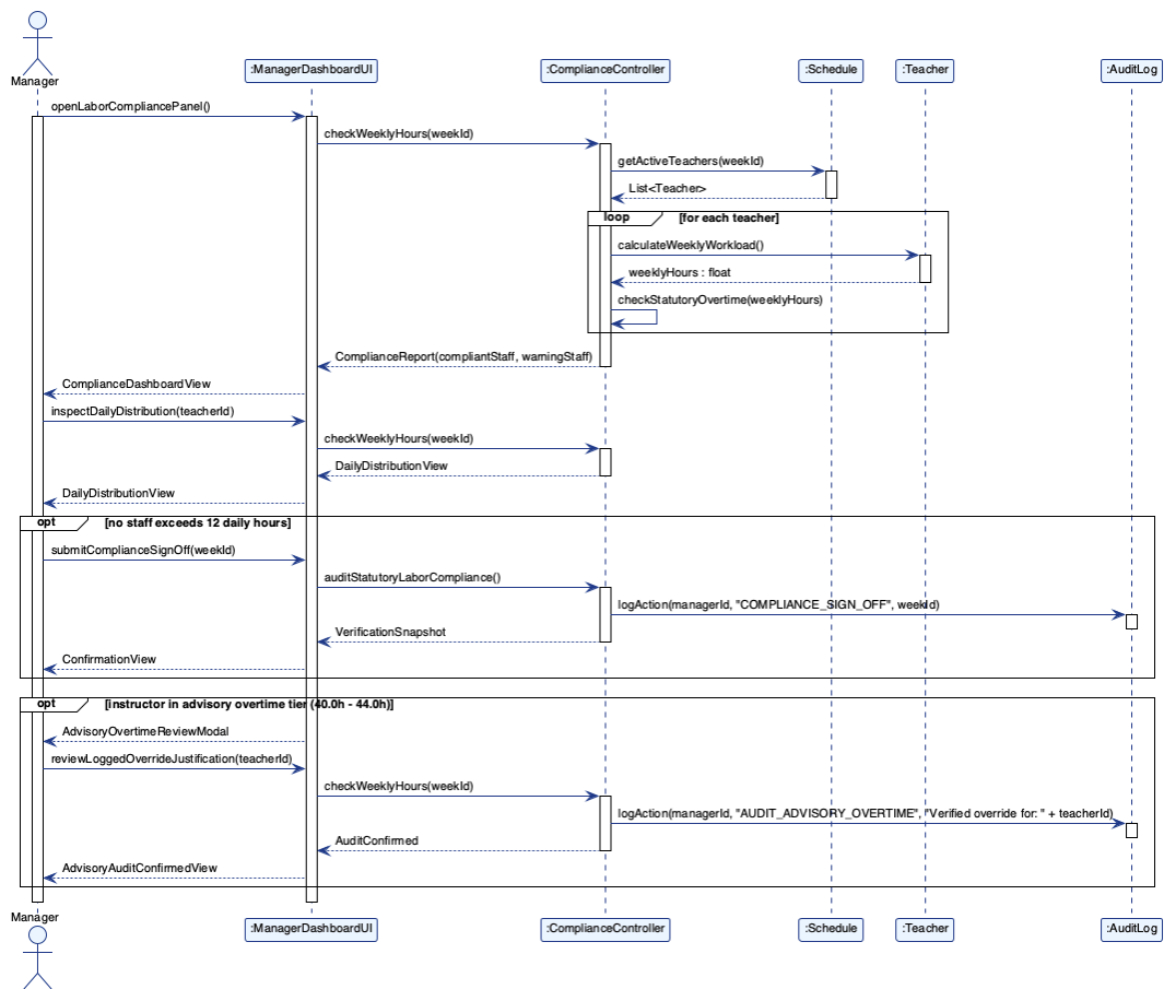
Figure 4.19: SSD-18 Review Labor Compliance & Workload
