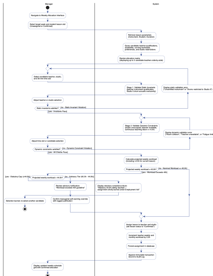
Figure 3.2: Activity Diagram for Weekly Job Allocation Workflow
