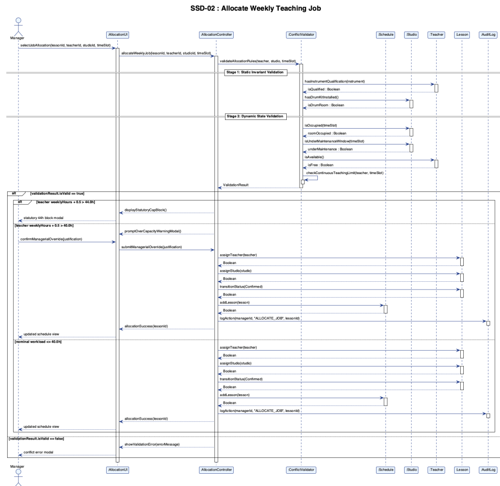
Figure 4.4: SSD-02 Allocate Weekly Teaching Job
