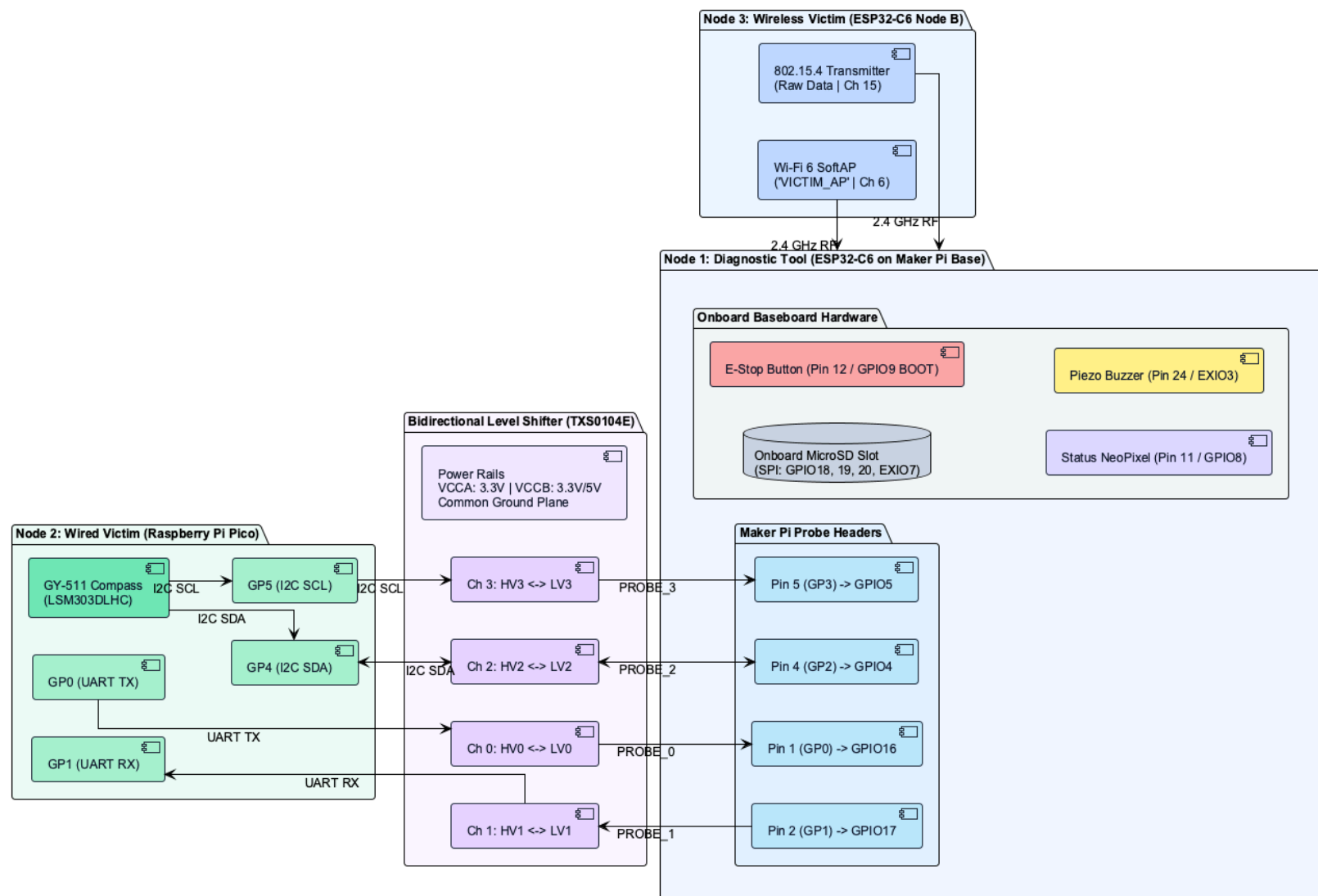
Figure 1: Hardware Interconnect & Maker Pi Base Pinout
