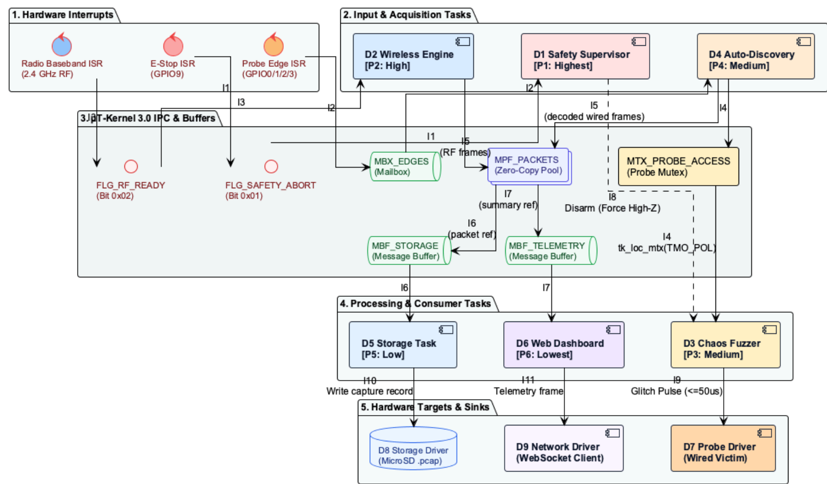
Figure 2: \mu T-Kernel 3.0 Task Interaction & IPC Architecture
