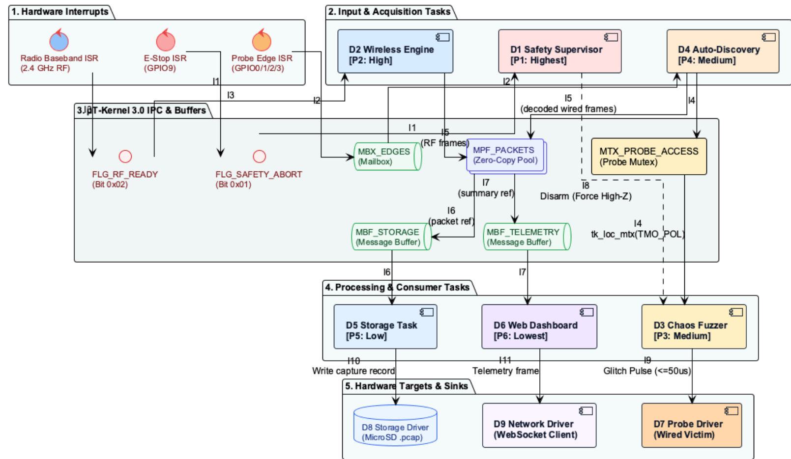
Figure 2: \mu T-Kernel 3.0 Task Interaction & IPC Architecture
