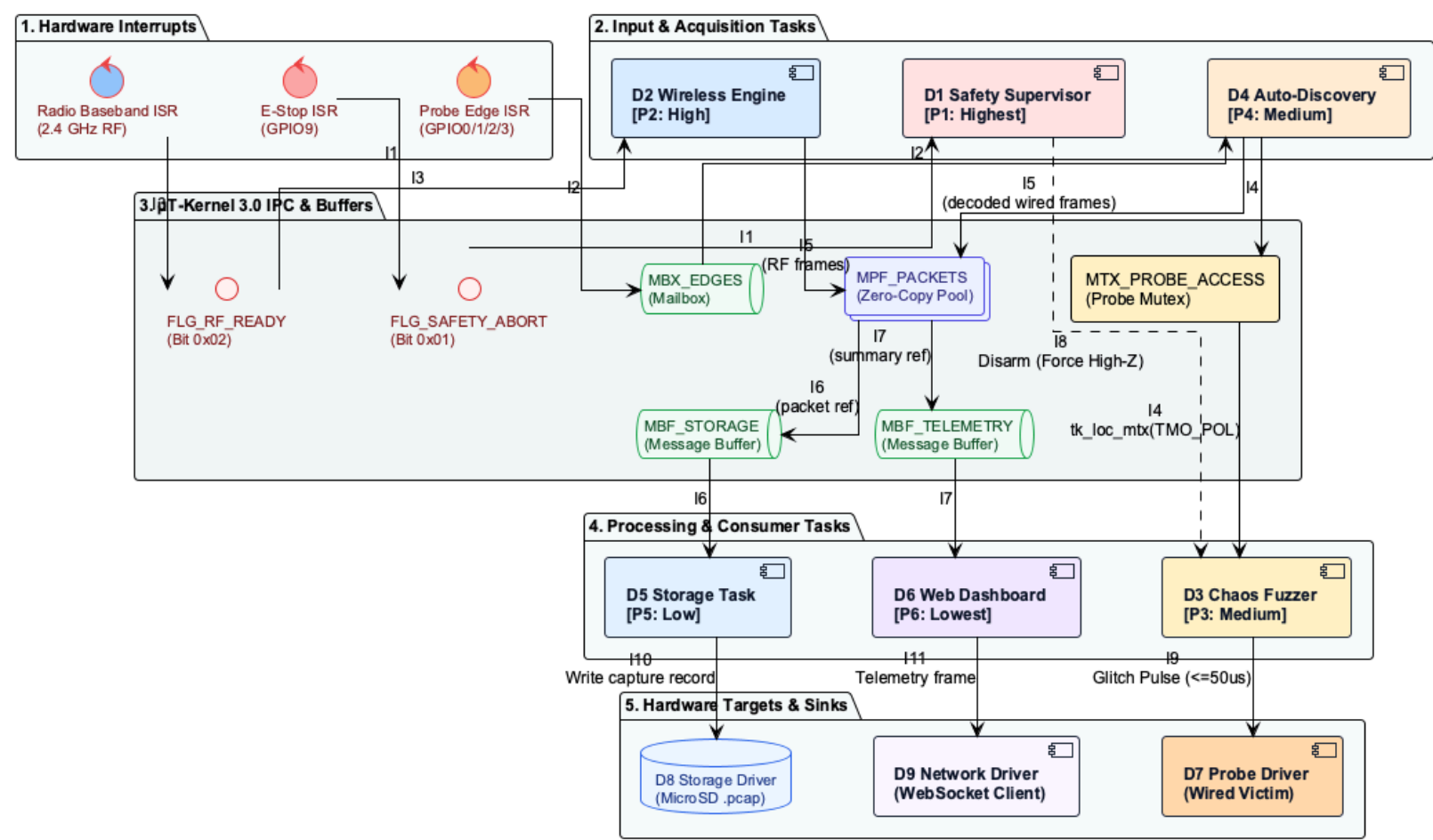
Figure 2: μT-Kernel 3.0 Task Interaction & IPC Architecture
