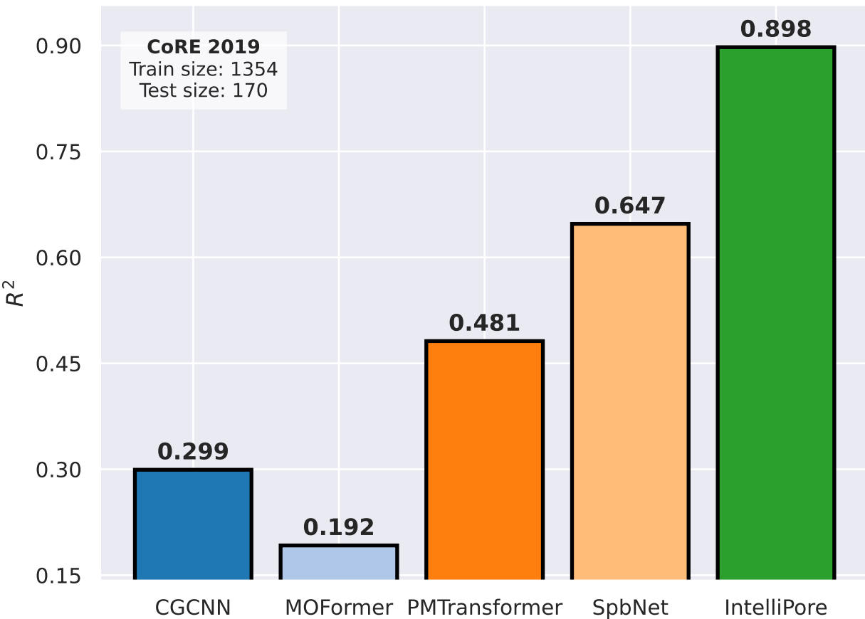
\text{C}_3\text{H}_6 log Henry coefficient at 298 K (MOFs)
