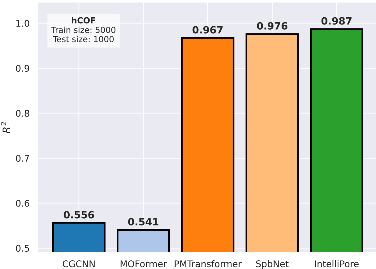
CH 4 uptake at 298 K and 65 bar (COFs)
