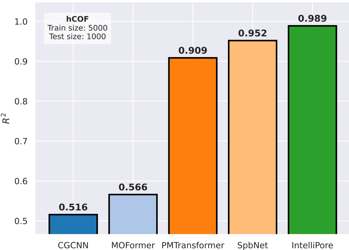
CH 4 uptake at 298 K and 5.8 bar (COFs)
