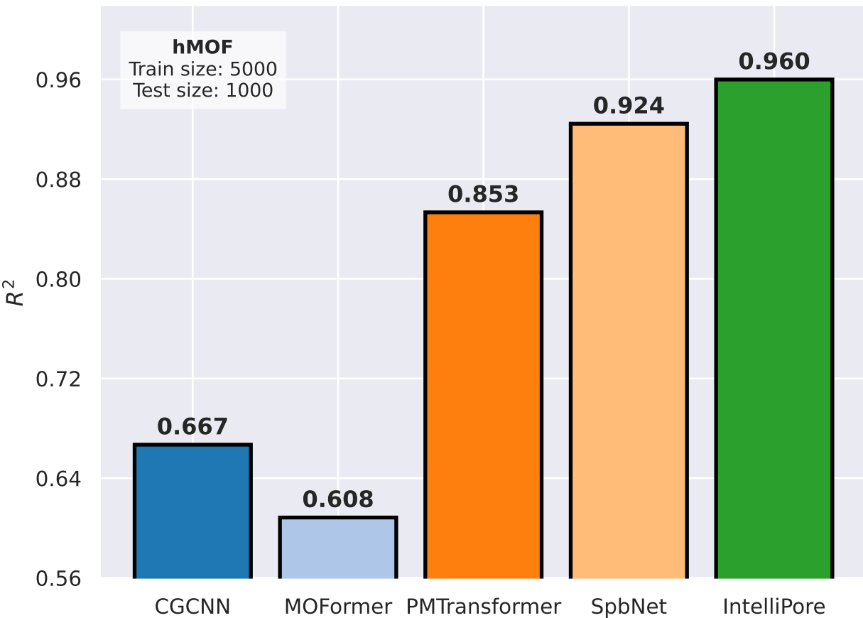
CH 4 uptake at 298 K and 2.5 bar (MOFs)
