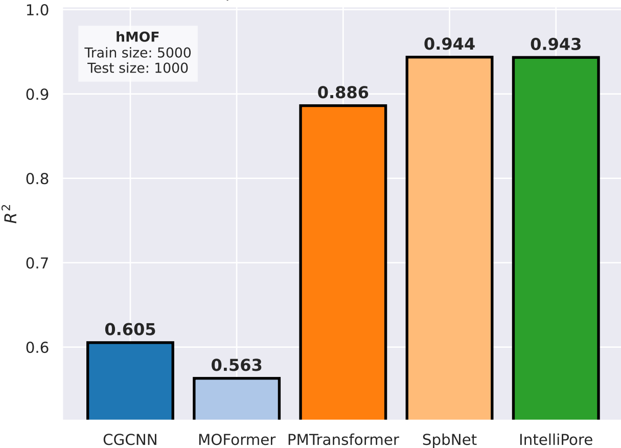
CO 2 uptake at 298 K and 2.5 bar (MOFs)
