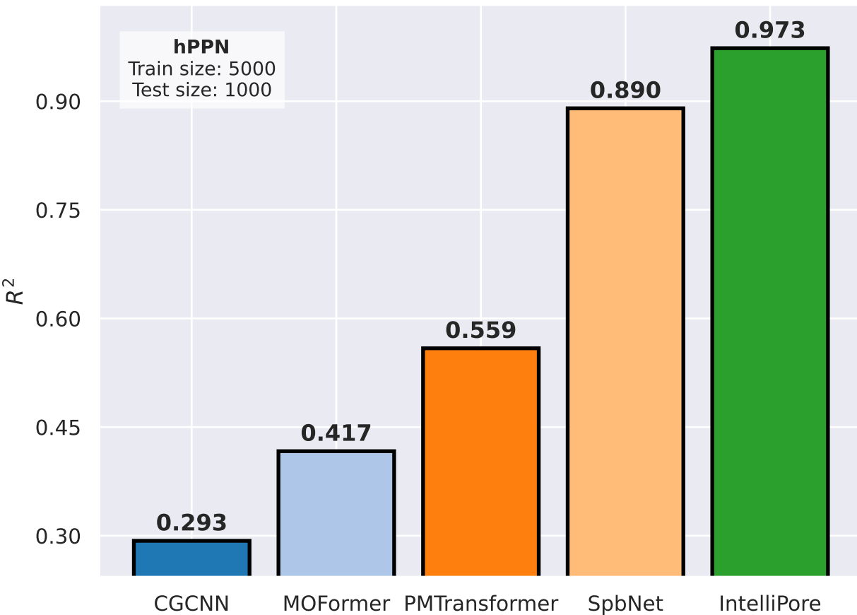
CH 4 uptake at 298 K and 1 bar (PPNs)
