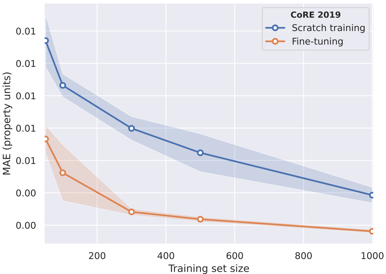
C_3H_8 (log) Henry coefficient at 298 K (MOFs)
