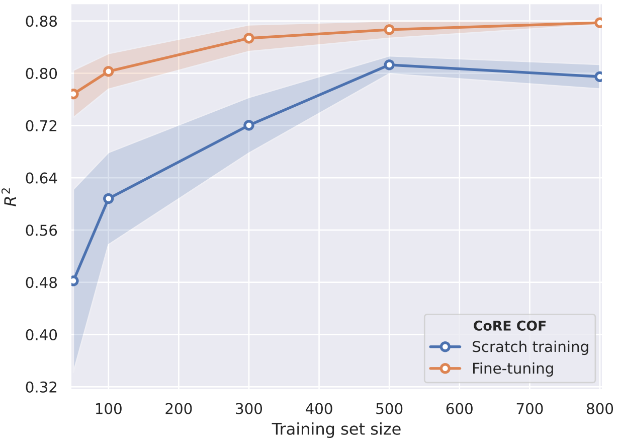
CO 2 log Henry coefficient at 298 K (COFs)
