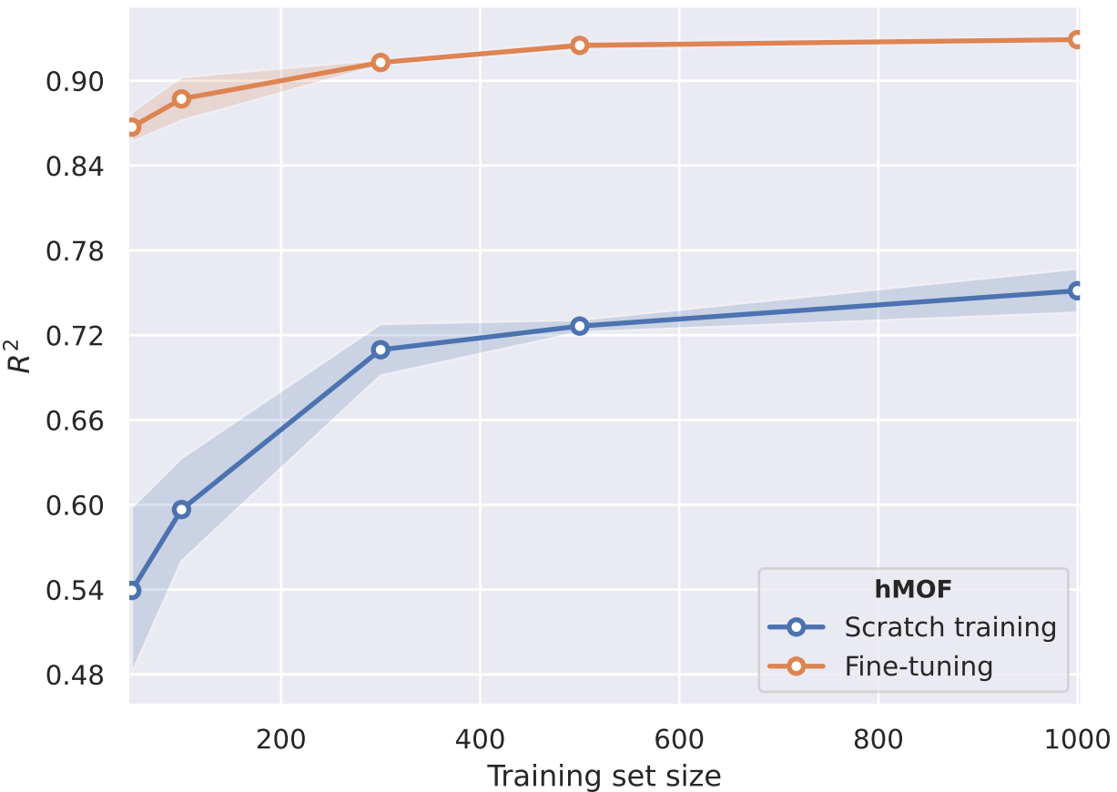
CO 2 uptake at 298 K and 2.5 bar (MOFs)
