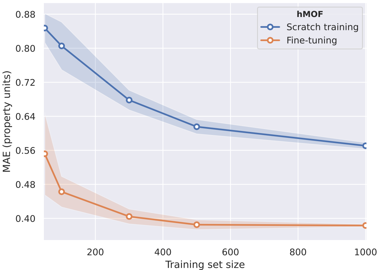
Kr binary uptake at 273 K and 10 bar (MOFs)
