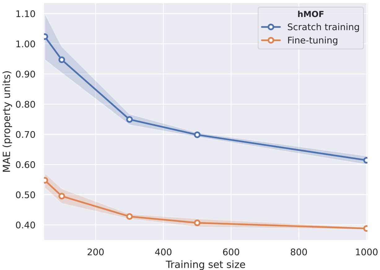
Xe binary uptake at 273 K and 10 bar (MOFs)
