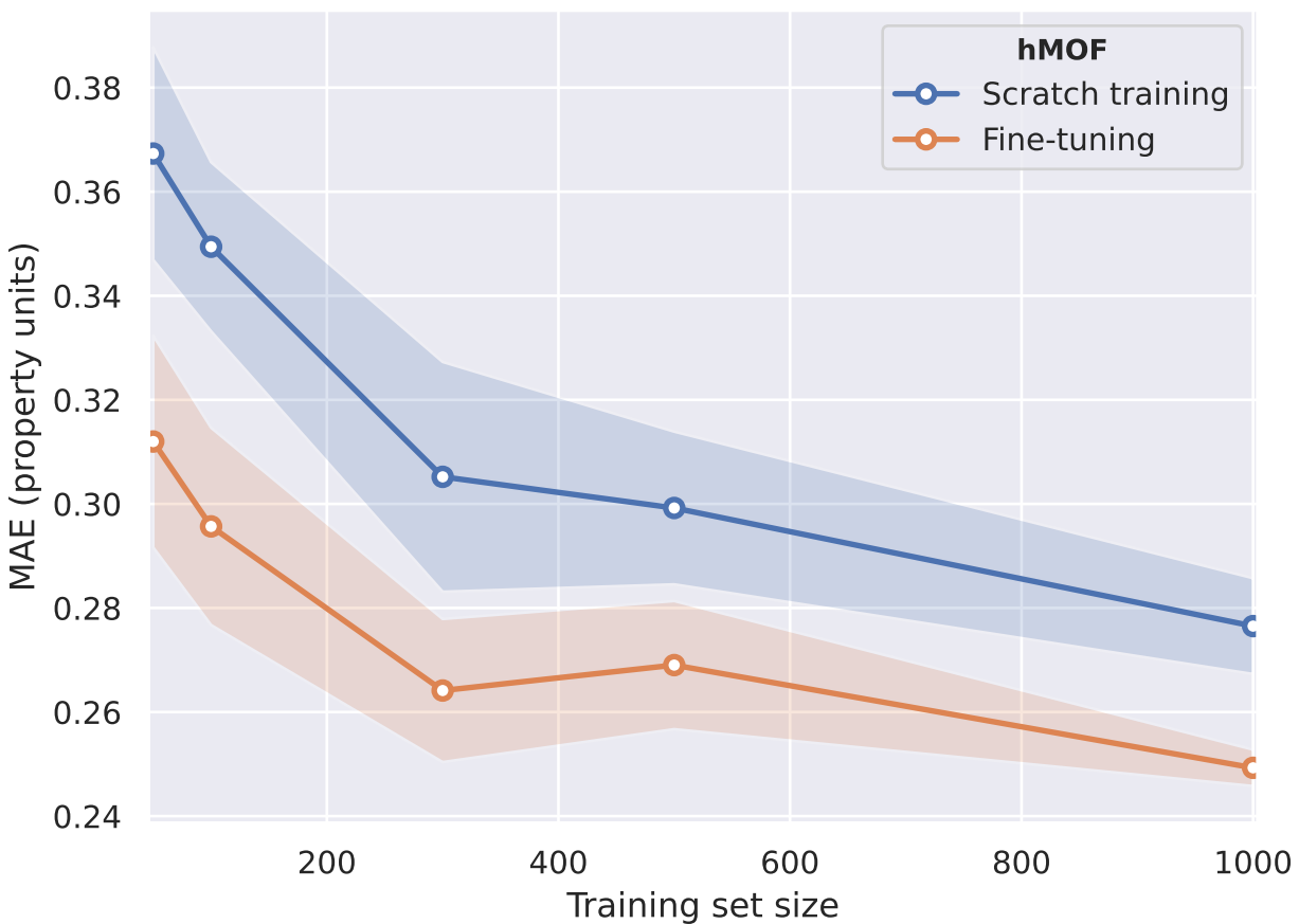
H 2 heat of adsorption at 77 K and 2 bar (MOFs)
