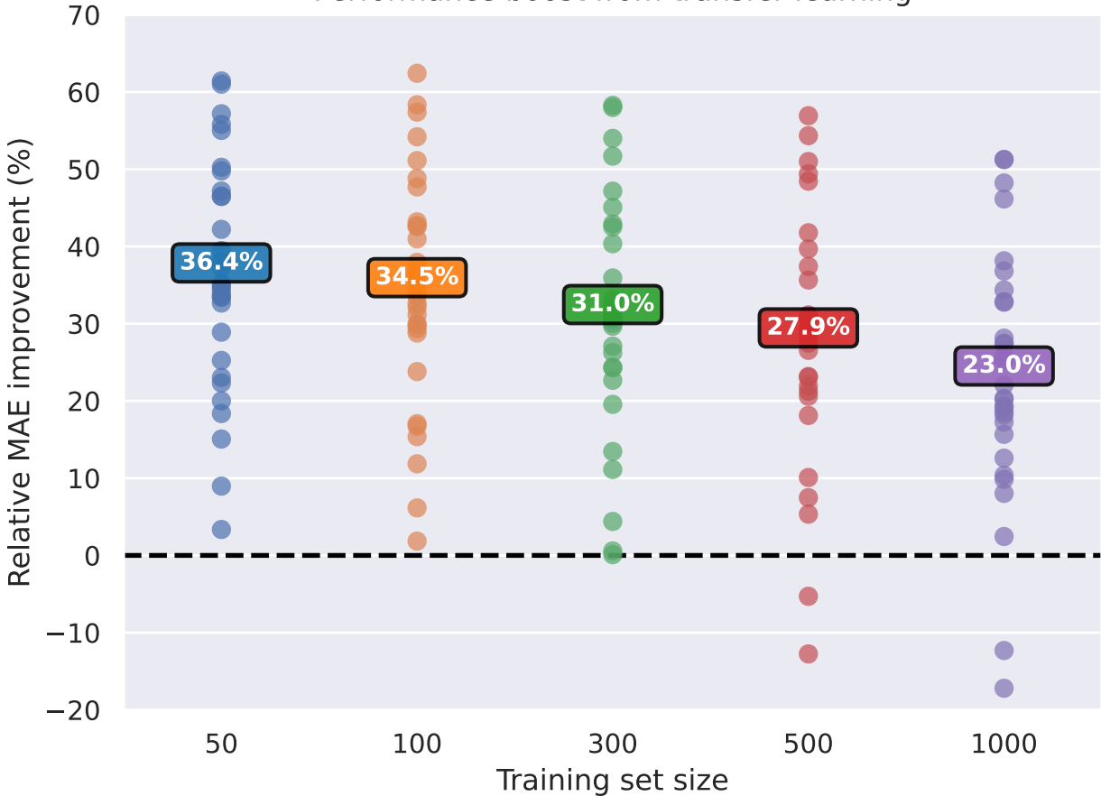
Performance boost from transfer learning
