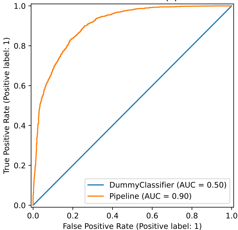
ROC curve of the best pipeline
