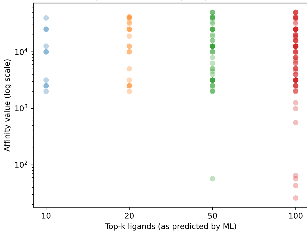
Affinity values for the top-k ligands of "1lox"
