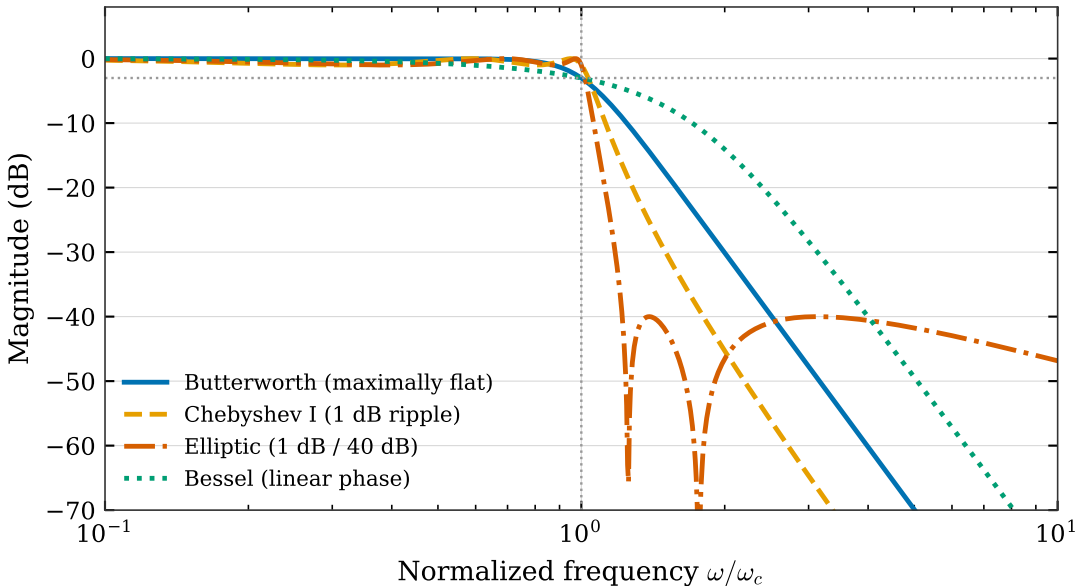
Order-5 low-pass filter families
