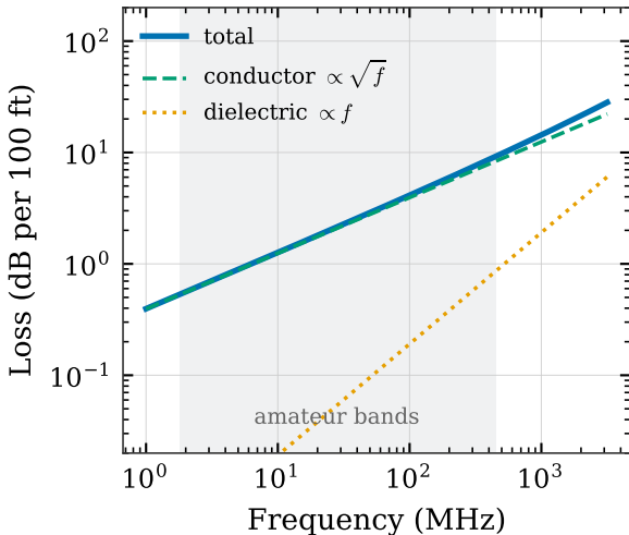
Two loss mechanisms (RG-58)
