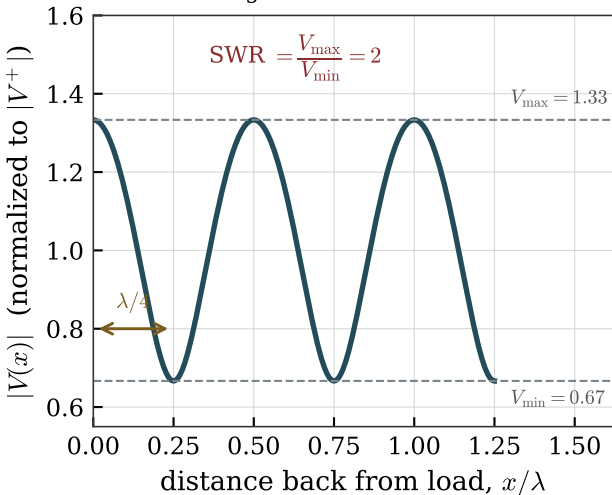
Standing wave: 100\,\Omega on a 50\,\Omega line
