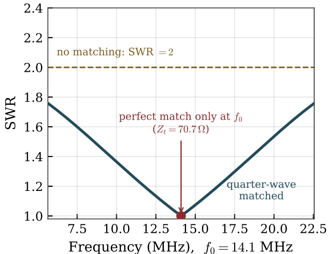
The match is narrowband
