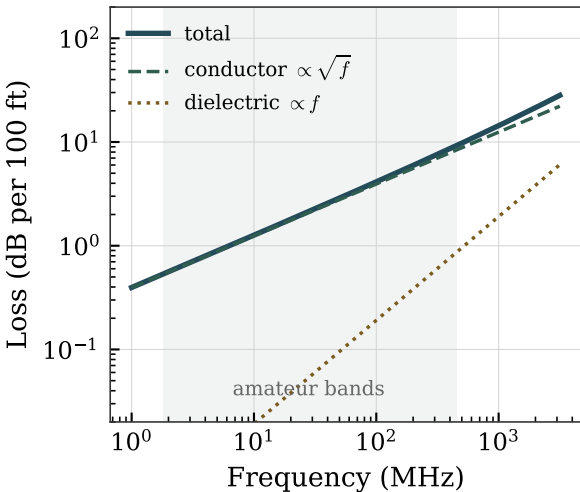
Two loss mechanisms (RG-58)
