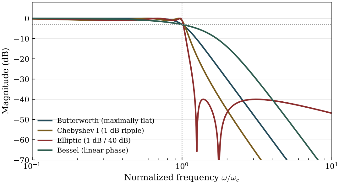
Order-5 low-pass filter families
