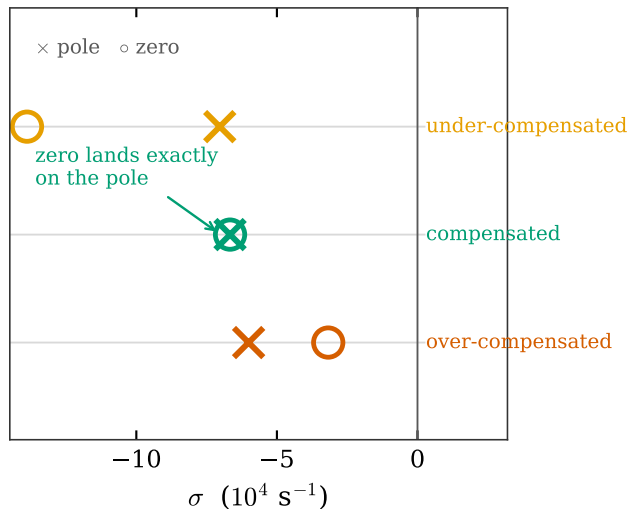
The same three cases in the s-plane
