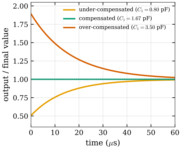
Step response through the probe
