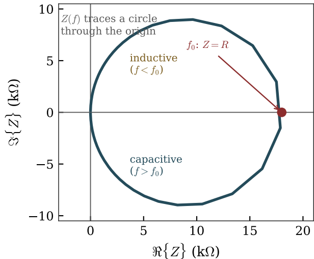
Z(f) in the complex plane
