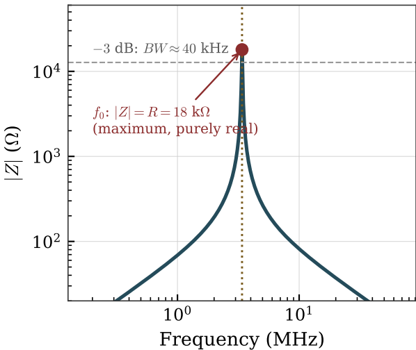
Tank impedance peaks at f_0
