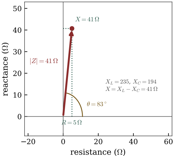
Z as a phasor at f = 1.1f_0
