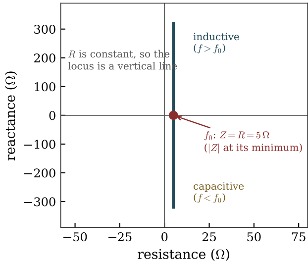
Z(f) sweeping through resonance
