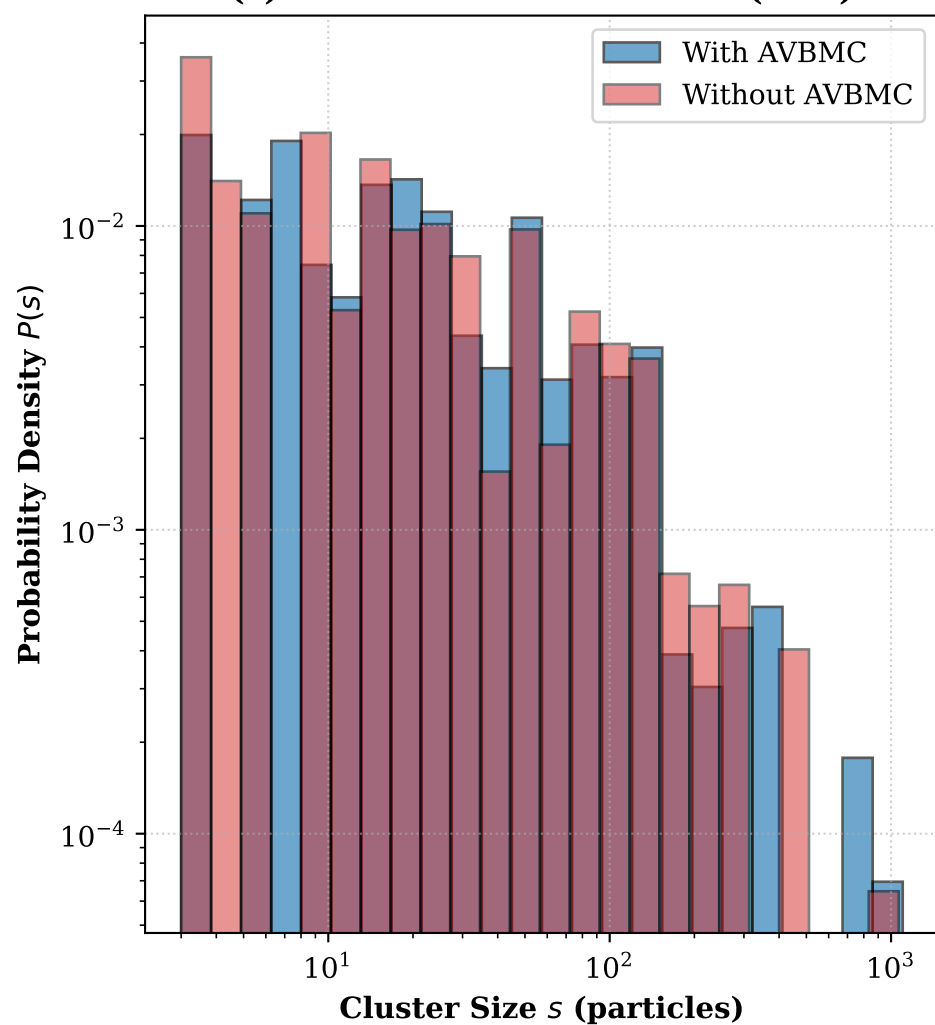
(c) Cluster Size Distribution (CSD)
