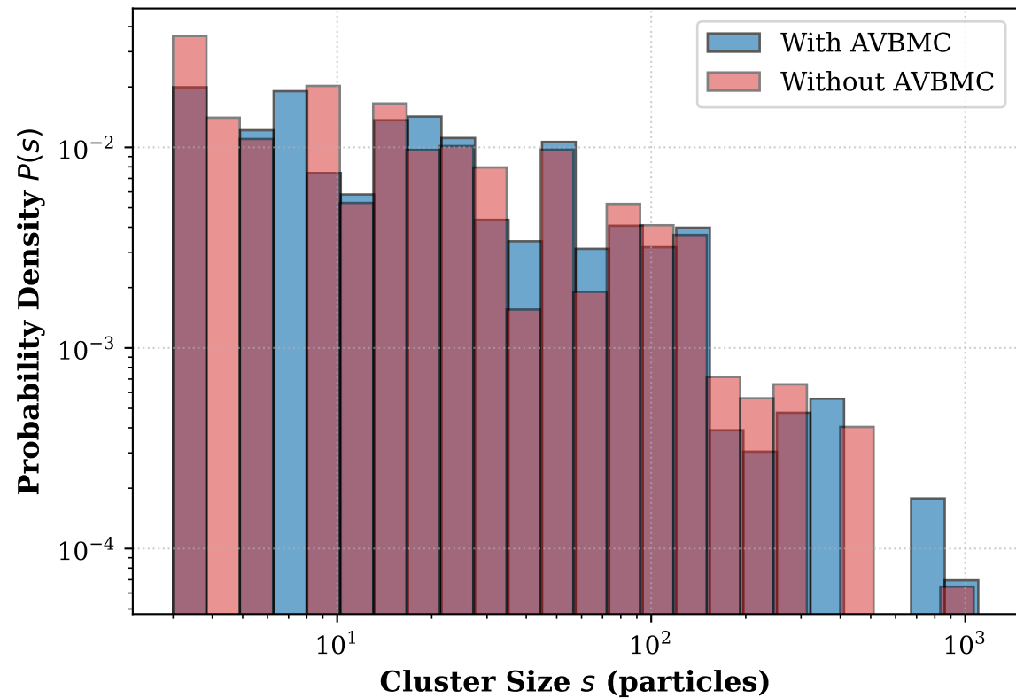
Cluster Size Distribution (CSD)
