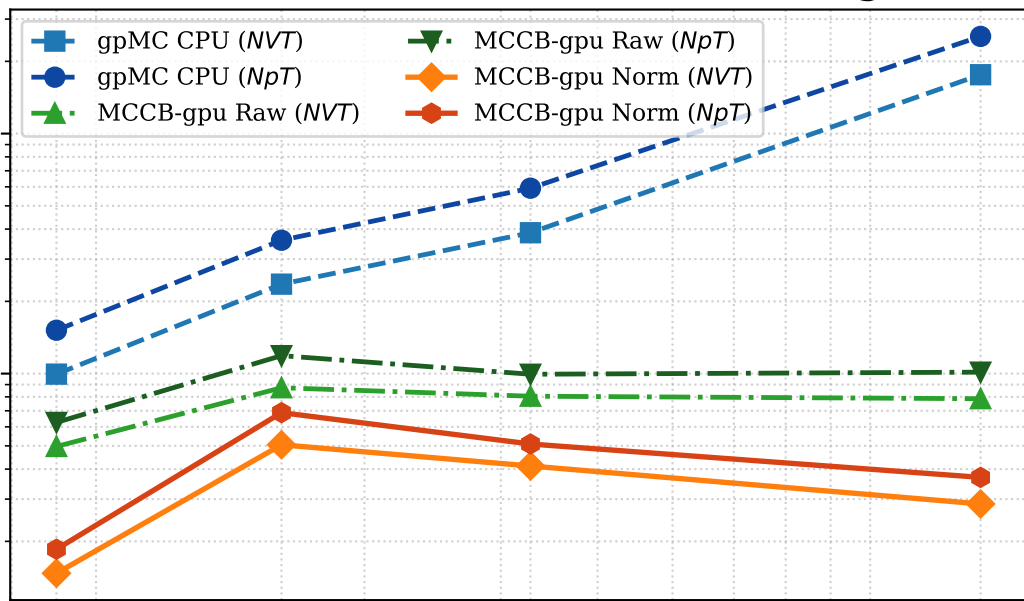
(a) Wallclock Execution Time Scaling
