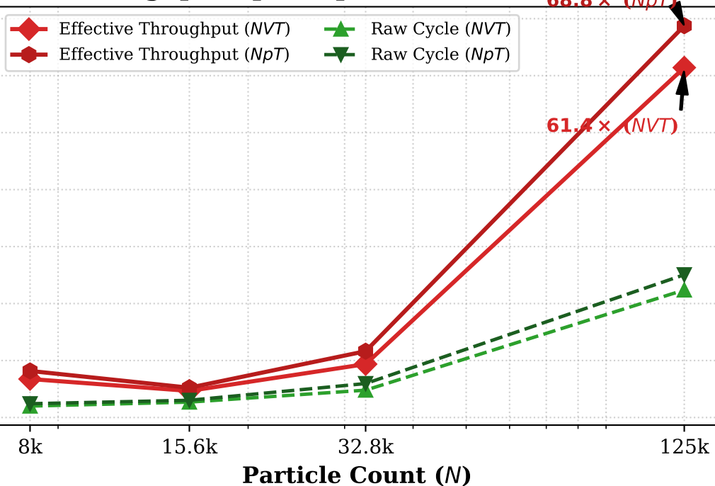
(b) Throughput Speedup Factor across Ensembles
