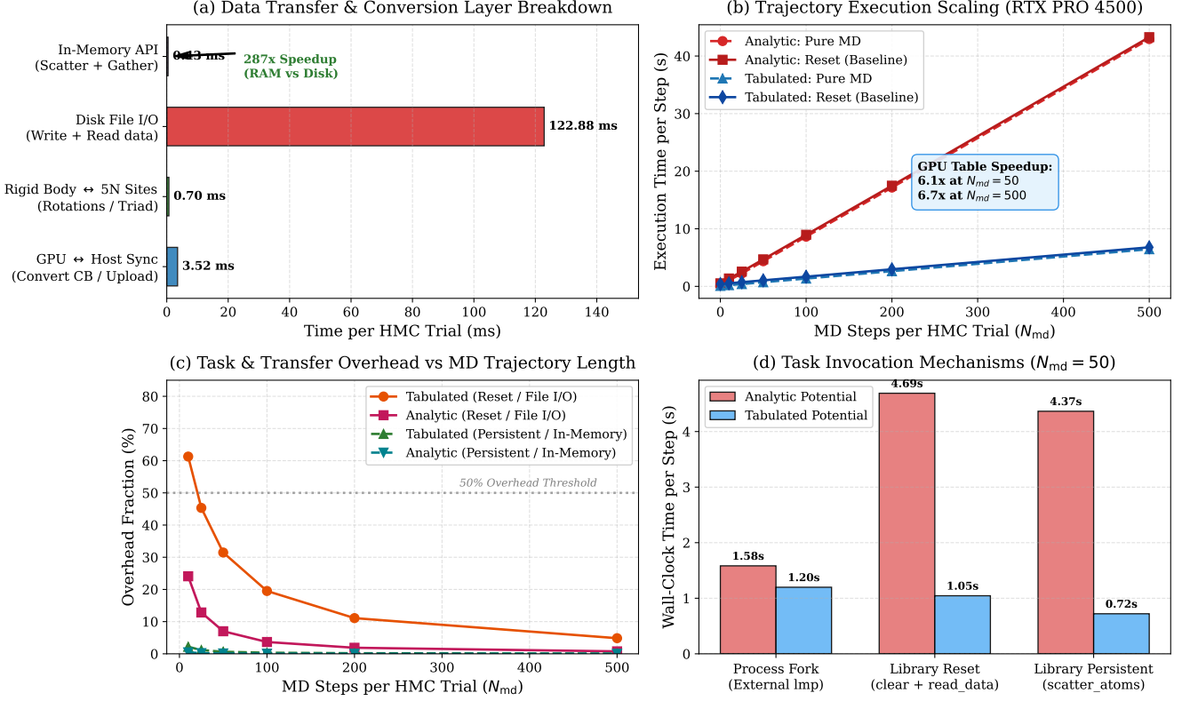
Figure 1: Profiling of In-Memory HMC Coupling with LAMMPS on NVIDIA RTX PRO 4500: (a) Latency breakdown showing the 287 \times speedup of direct in-memory C-API coordinate transfer (0.43 ms) over disk ASCII file I/O (122.9 ms). (b) MD trajectory propagation scaling with N_{\text{md}} , highlighting a 6.1 \times –6.7 \times throughput advantage for GPU-accelerated tabular potentials over analytic overlays. (c) Coupling overhead fraction versus N_{\text{md}} . (d) Comparison of task invocation paradigms for N_{\text{md}} = 50 steps.
