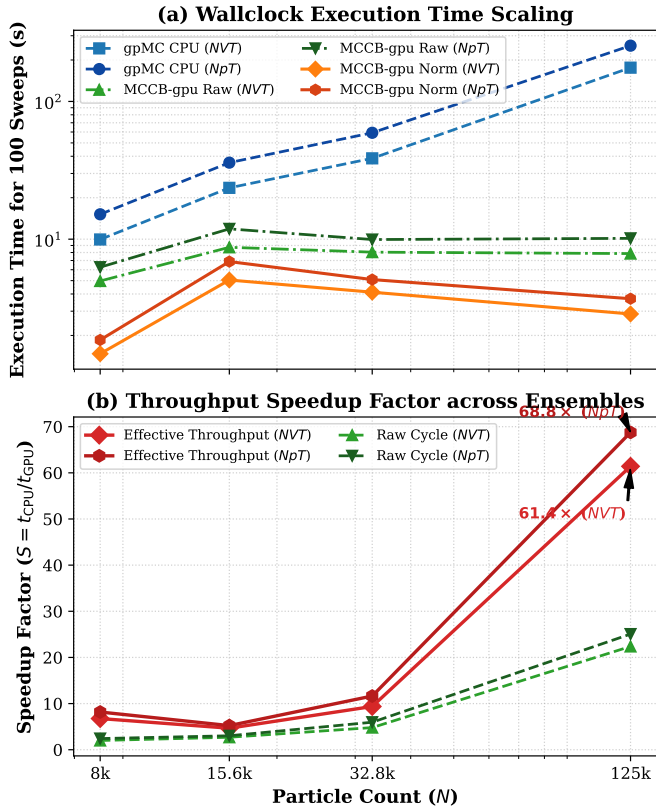
Figure 3: gpMC (CPU) vs. MCCB-gpu (GPU) Performance Scaling across NVT and NpT Ensembles: (a) Wallclock execution times for 100 sweeps on Intel Xeon Gold 6548Y+ vs. NVIDIA RTX PRO 4500. (b) Effective throughput speedup factor S_{eff} accounting for moves per particle, reaching 61.4 \times in NVT and 68.8 \times in NpT .
