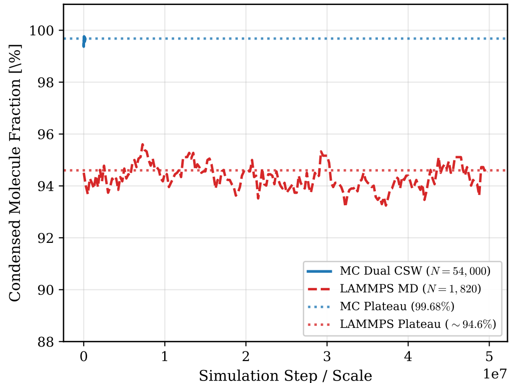
Condensed Fraction Evolution
