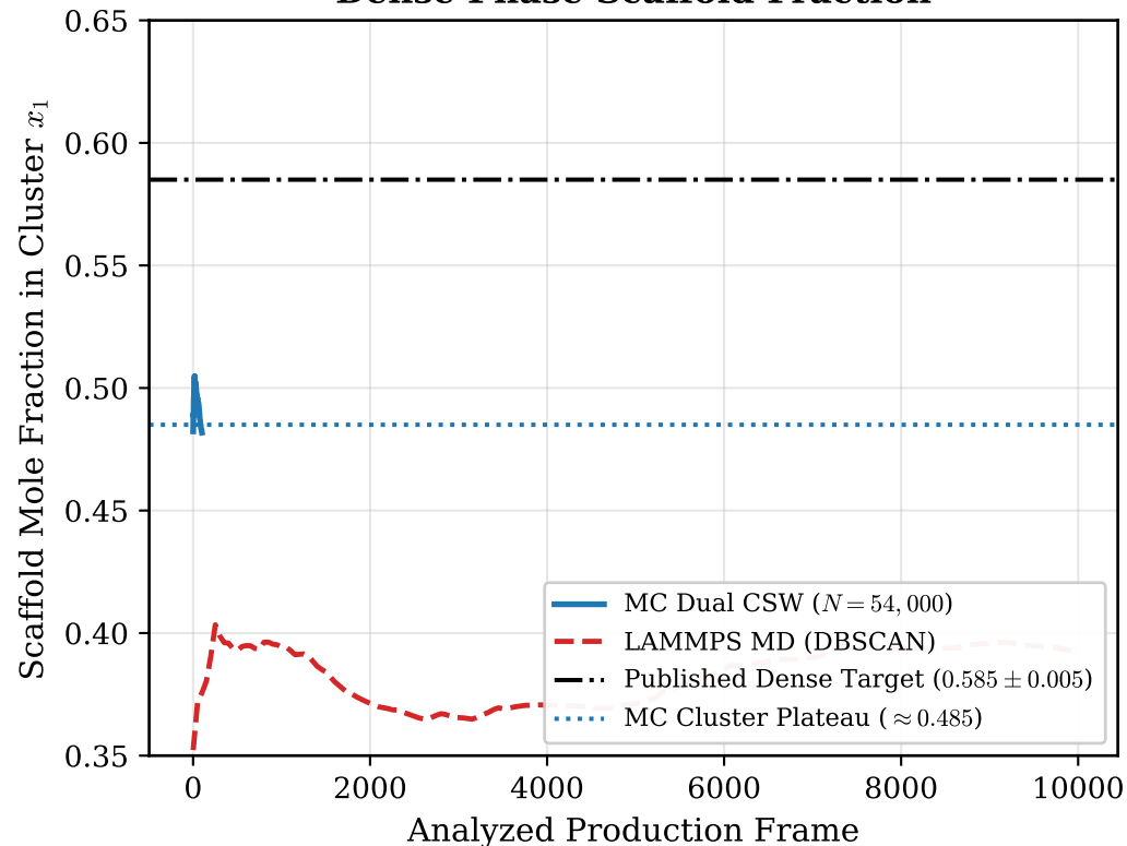
Dense Phase Scaffold Fraction
