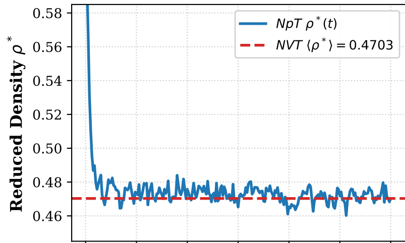
(b) Lennard-Jones (LJ)
