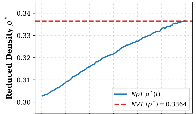
(a) Hard Spheres (HS)
