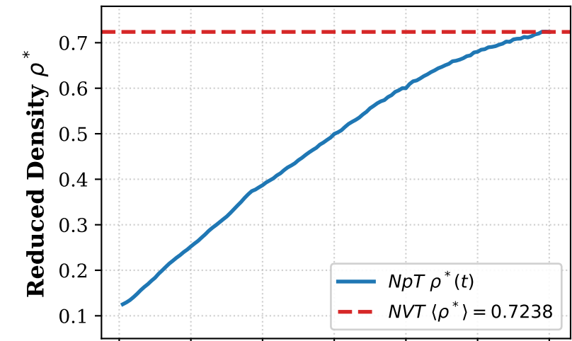
(c) Site-Site Patchy (SSP)
