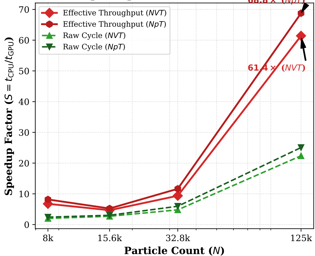
(b) Speedup Factor across Ensembles
