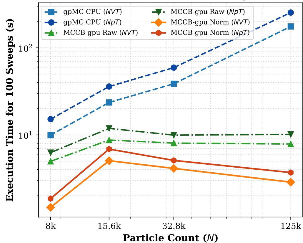
(a) Execution Time Scaling
