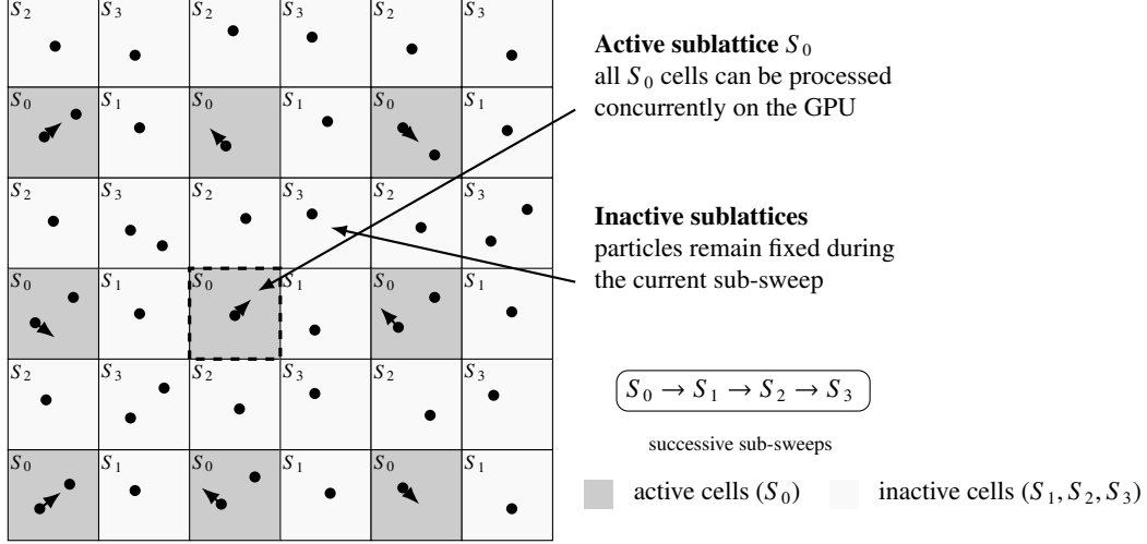
Figure 1: Schematic representation of the four-sublattice checkerboard Monte Carlo algorithm in two dimensions.
