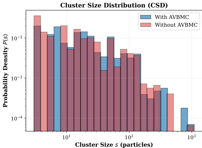
Figure 6: Final Cluster Size Distribution (CSD) for Patchy Colloids With vs. Without AVBMC: Normalized probability P(s) versus cluster size s after 200 sweeps, highlighting that AVBMC significantly accelerates aggregation into large macromolecular clusters ( s > 500 ) compared to kinetically arrested canonical sampling.
