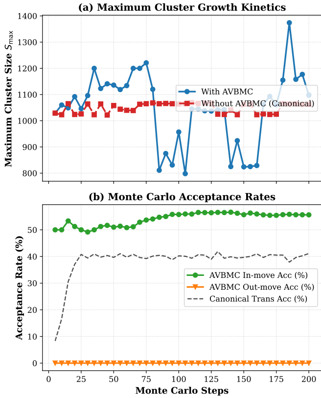
Figure 5: Comparative Benchmark of Patchy Colloidal Cluster Sampling With vs. Without AVBMC: (a) Maximum cluster size evolution S_{\max}(t) demonstrating accelerated aggregation kinetics and overcoming kinetic traps. (b) Monte Carlo acceptance rates for association ( P_{\text{AV},\text{in}} ), dissociation ( P_{\text{AV},\text{out}} ), and standard canonical displacement ( P_{\text{trans}} ), sharing the Monte Carlo simulation steps coordinate.
