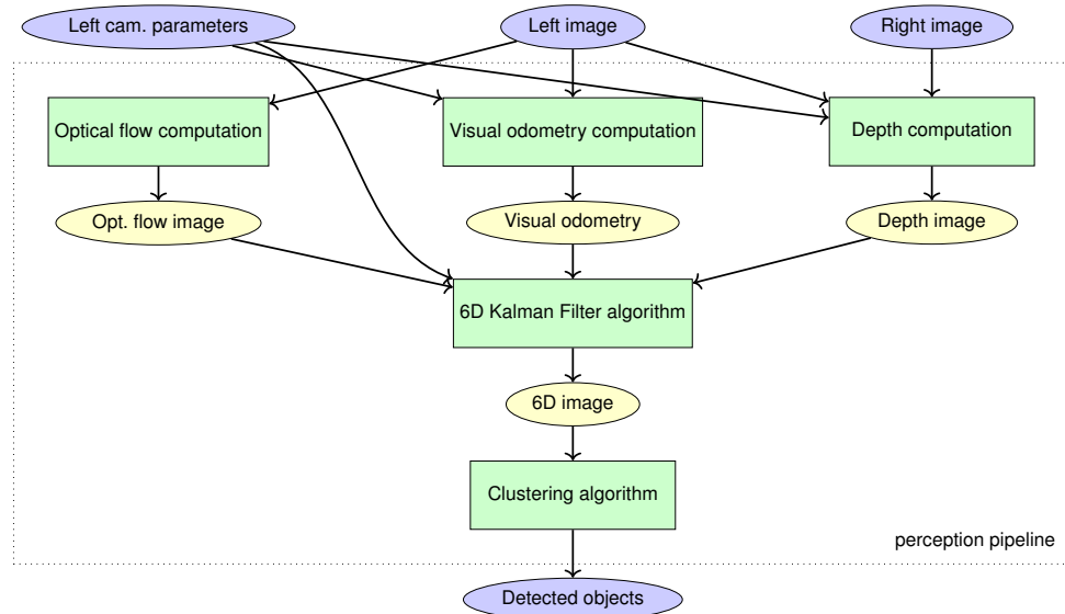
Abbildung 3.3: High level perception pipeline
