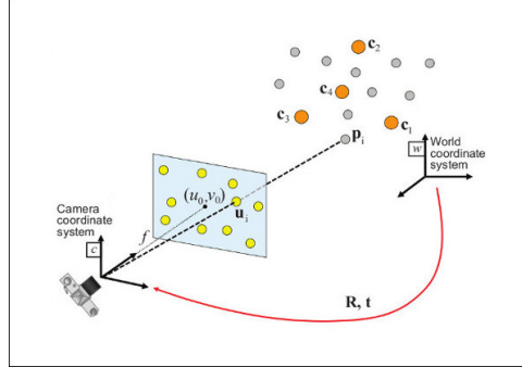
Abbildung 3.16: Perspective-n-Point (PnP) problem. Source: [63]
