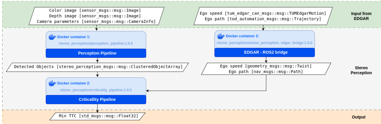
Abbildung 3.5: Container architecture and data flow
