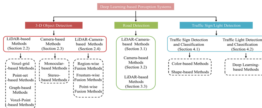
Abbildung 2.1: Learning-based perception methods. Source: [15]
