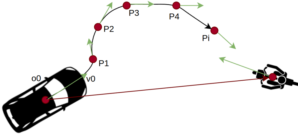
Abbildung 3.30: Time-to-collision with ego path consideration. Source: own work
