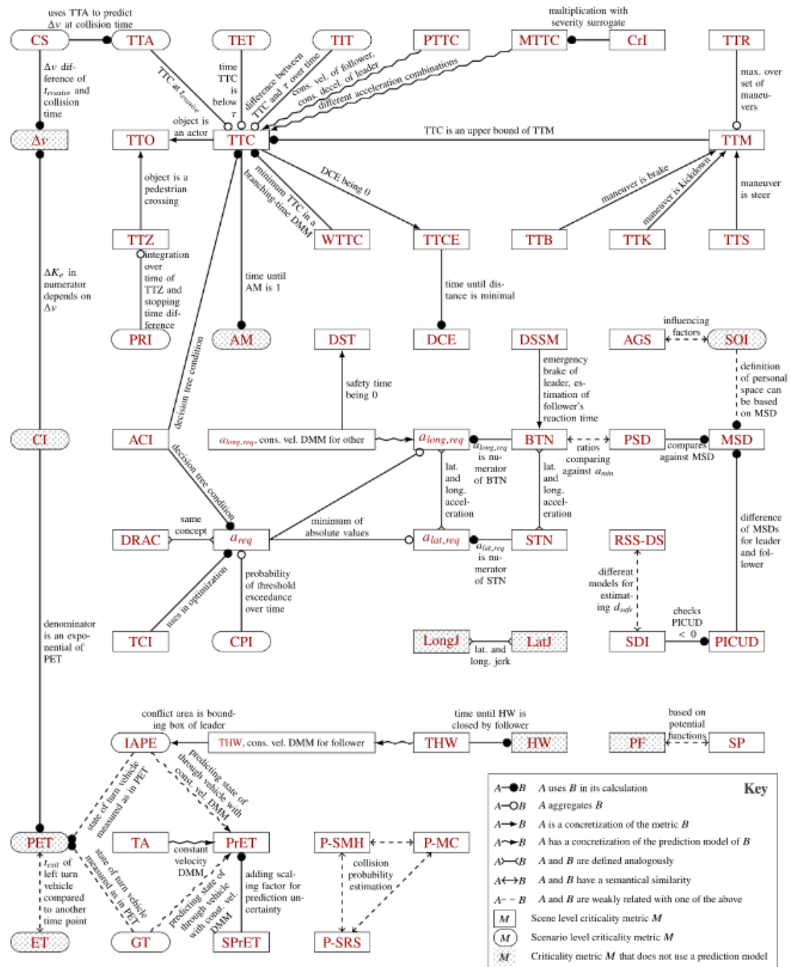
Abbildung 3.27: Dependency graph of criticality metrics based on TTC. Adapted from [38].
