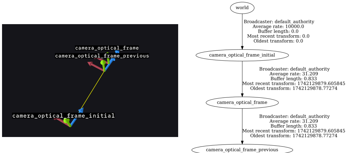
Abbildung 3.13: Coordinate frames and ROS2 TF tee. Left: Coordinate frames visualized using Foxglove. Right: ROS2 Transform Tree of the project generated using tf2_tools. Source: own work
