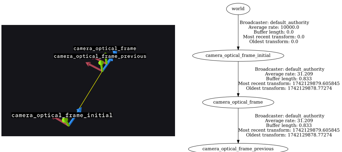
Figure 3.12: Coordinate frames and ROS2 TF tree. Left: Coordinate frames visualized using Foxglove. Right: ROS2 Transform Tree of the project generated using tf2_tools. Source: own work
