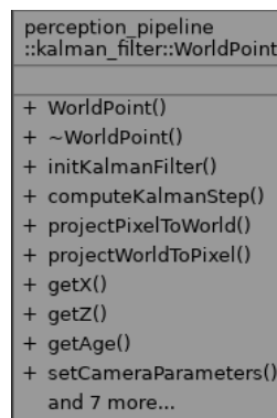
Figure 3.18: WorldPoint class. Source: own work
