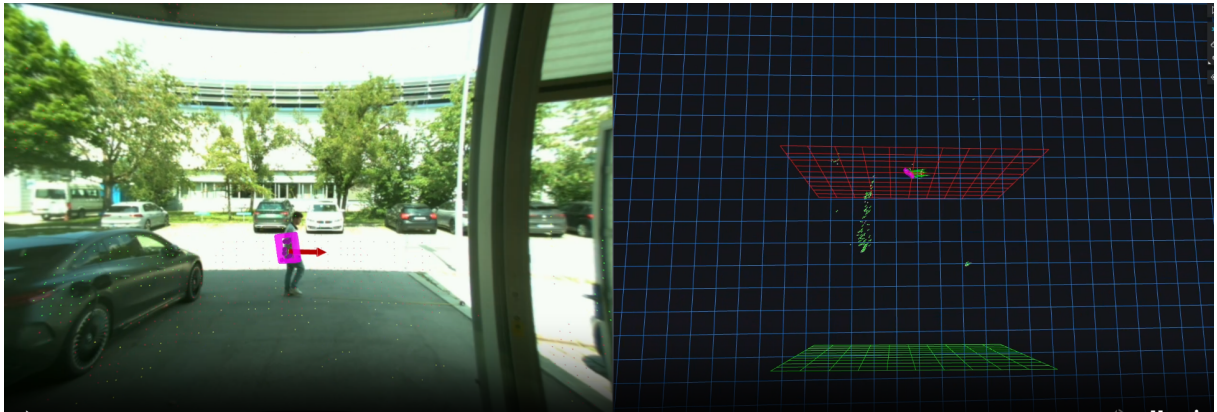
Figure 4.11: Lateral motion test: return traversal from left to right.
