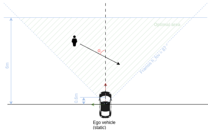
Figure 4.6: Angle test experiment setup. Source: own work
