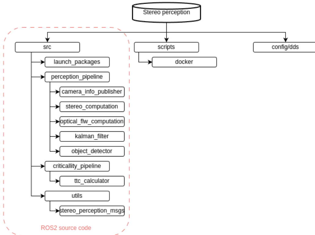
Abbildung 3.5: Overview of the repository structure
