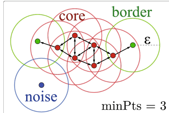
Abbildung 3.23: Illustration of DBSCAN clustering: core, border, and noise points. Source: [72]
