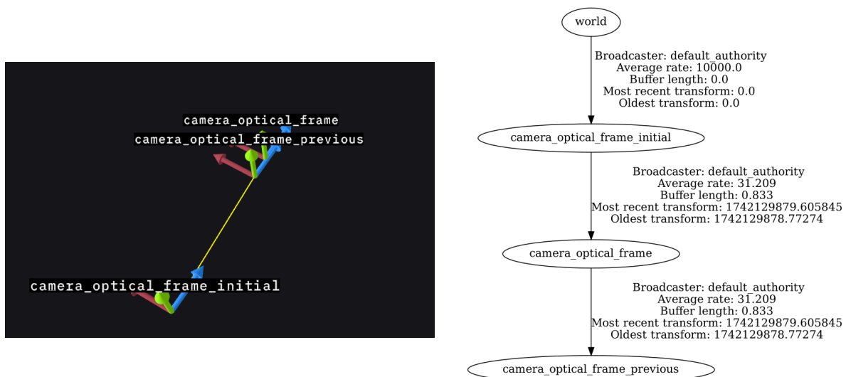
Abbildung 3.13: Coordinate frames and ROS2 TF tee. Left: Coordinate frames visualized using Foxyglove. Right: ROS2 Transform Tree of the project generated using tf2_tools. Source: own work
