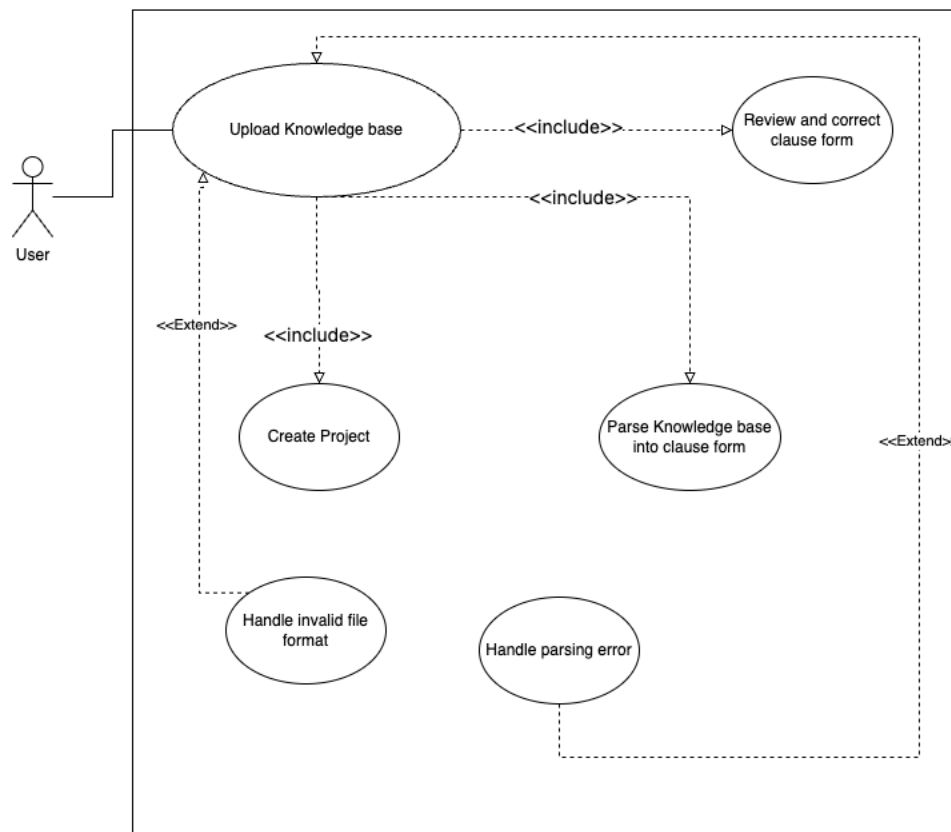
Upload a knowledge base Use Case Diagram
