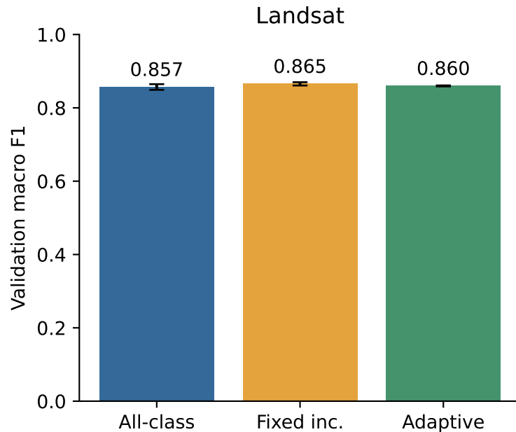
Pilot only: mean \pm sample SD over 3 optimisation seeds
