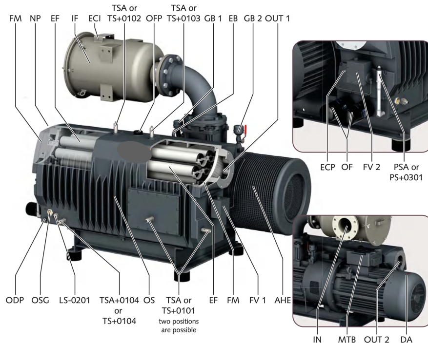
Figure 2.8: Vacuum pump scheme. Adapted from Sysadvance
