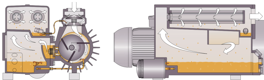
Figure 2.7: Vacuum pump operating principle. Adapted from Sysadvance
