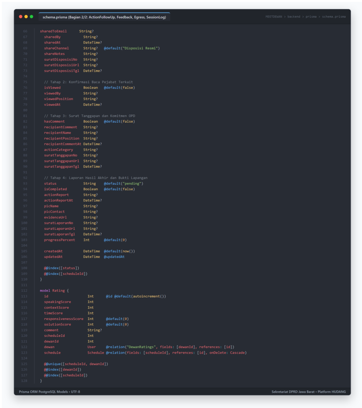
Gambar 4.4b: Cuplikan Skema Relasional Prisma (Bagian 2: ActionFollowUp, Feedback, Egress, SessionLog)
