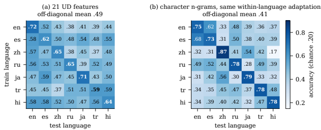
Figure 2. Cross-language transfer: a classifier trained on one language (rows) is tested on another (columns) after within-language z-scoring; the diagonal is LOPO within language. (a) UD features. (b) Character n -grams given the same adaptation (union vocabulary, TF-IDF columns z-scored per language).
