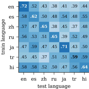
(a) 21 UD features off-diagonal mean .49
