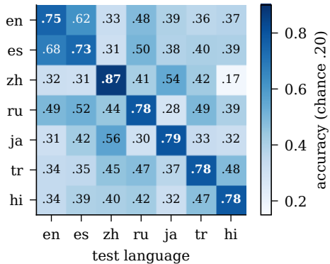
(b) character n-grams, same within-language adaptation off-diagonal mean .41
