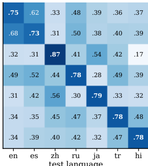
(b) char n-grams, adapted off-diagonal mean .41
