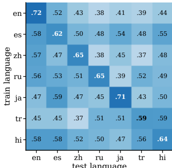
(a) UD features off-diagonal mean .49
