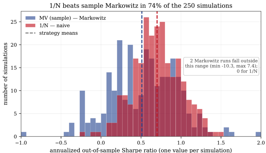
Figure 2: Distribution of the out-of-sample Sharpe ratio across the 250 simulations for 1/N (red) and the sample Markowitz rule (blue). The Markowitz distribution shows both a leftward shift
