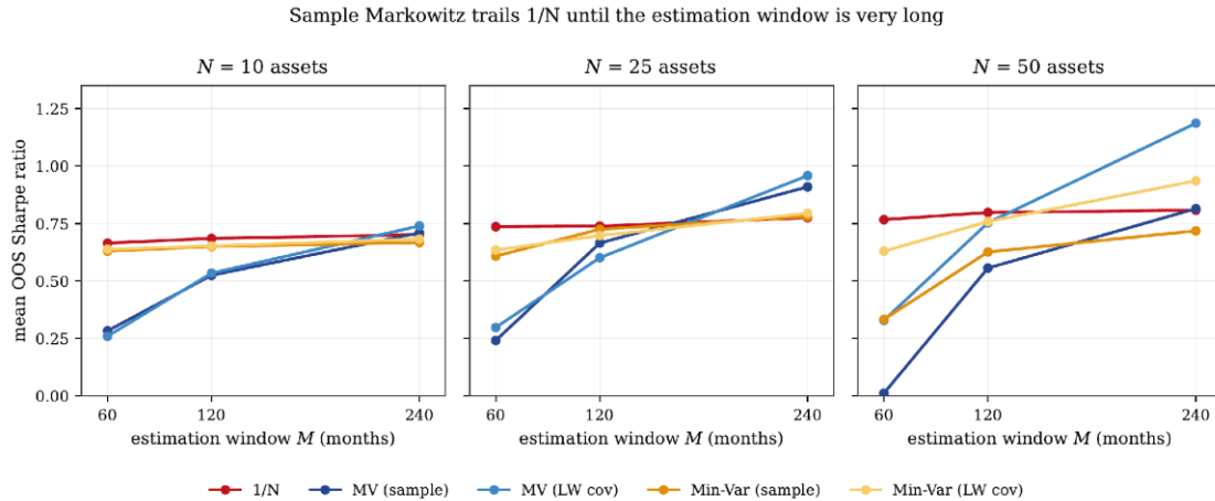
Figure 5: Out-of-sample Sharpe ratio versus estimation-window length M , for N = 10, 25, 50 assets (all panels share a common vertical scale). Sample Markowitz (dark blue) starts far below 1/N (red) and climbs as more data become available, reaching 1/N only around a 20-year window. The collapse at short windows worsens sharply with N —at N = 50 , M = 60 the sample optimizer is essentially worthless—which is precisely the regime where Ledoit–Wolf shrinkage (light blue) rescues it. Minimum-variance rules (orange) sit close to 1/N throughout because they never estimate expected returns.
