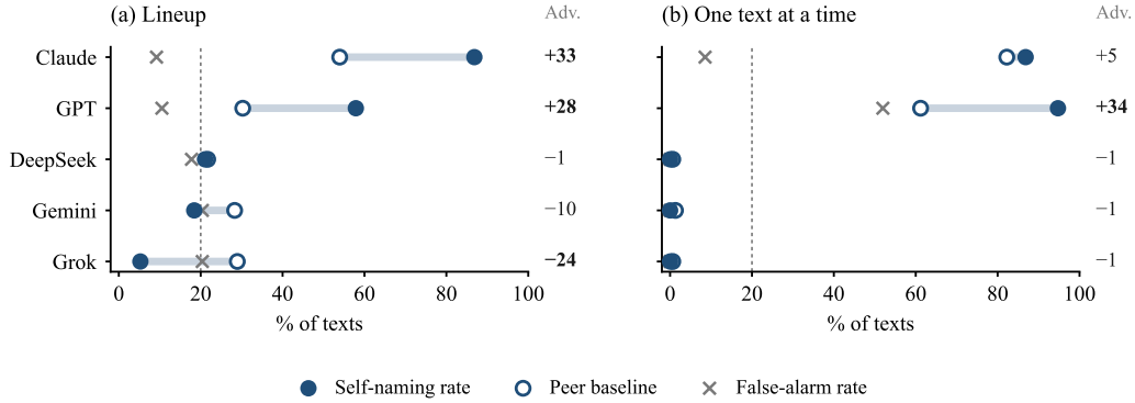
Figure 1: The same self-naming rate (filled circle) can mean very different things. Read it against the peer baseline (open circle: how often the other four judges name this judge on its text) and the false-alarm rate ( \times : how often the judge names itself on text it did not write). Five frontier judges, 38 essays each; the numbers on the right are the self-advantage in percentage points; the dashed line is the 20% chance level. In the lineup, Claude and GPT beat their peers and Grok trails them. Shown the same essays one at a time, three judges never name themselves, and Claude’s peers name Claude almost as often as Claude does.
