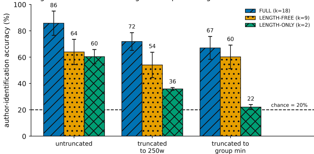
Engine A: how much of the signal is response length?
